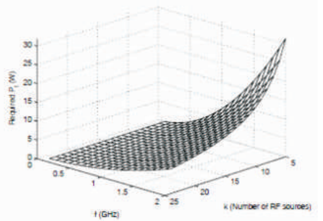
Figure 4: Required RF power for number of RF sources and frequency.
