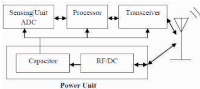
Figure 1: Structure of basic WPSN Node
