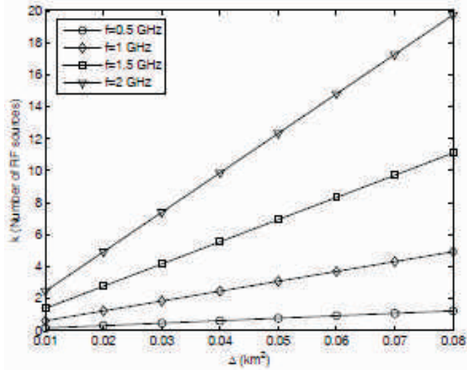
Figure 5: Variation of k with respect to the area of the event field
