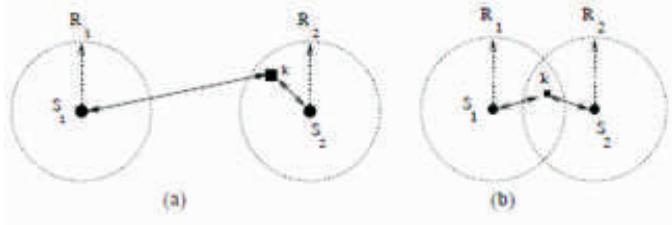
Figure 2: (a) Source-to-Source interference (b) Source-to-Node interference
