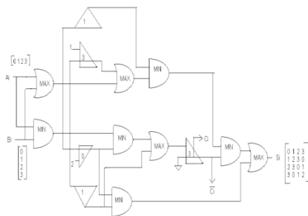
Figure 4.7: Voltage-Mode Quaternary Half-Adder
