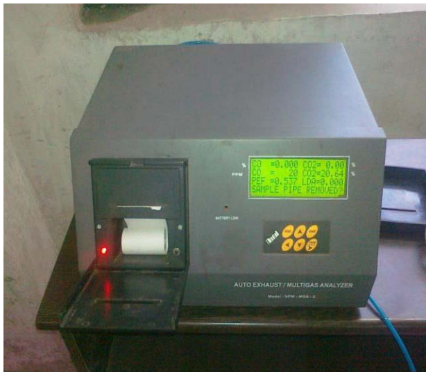
Fig. 1: Multi Gas Analyzer
