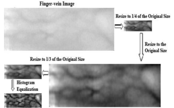
Fig.6. The procedure of our method for image enhancement
