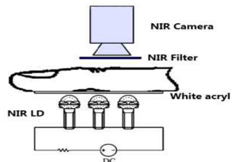
Fig. 2. Illustration of the imaging device
