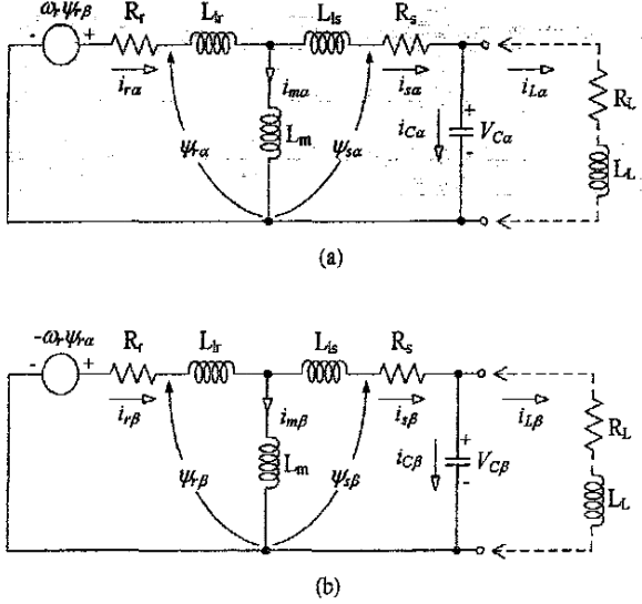
Fig.2. Equivalent Circuit of SCIM (a) \alpha axis (b) \beta axis
