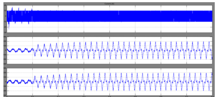
Fig. 18. Currents Response of Induction Motor Under Fault Condition
