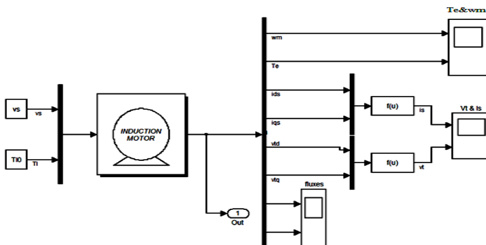
Fig. 5. Simulation Diagram of Induction Motor Under Open Circuit Condition
