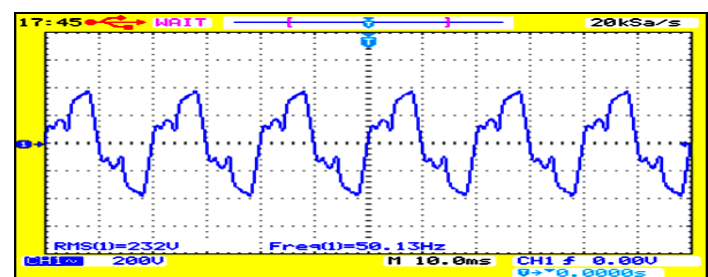
Fig. 21 Experimental Result for Voltage under Single Phasing Condition
