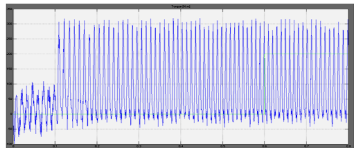
Fig. 17. Torque Response of Induction Motor Under Fault Condition
