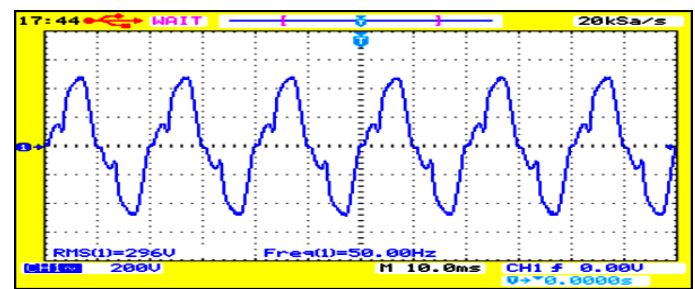
Fig 20. Experimental Result for Voltage under Normal Condition
