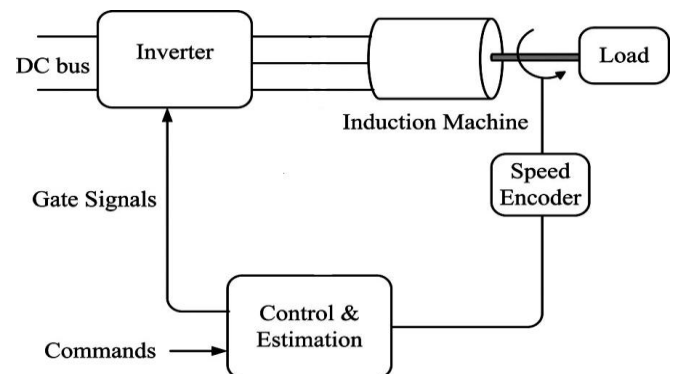
Fig. 1. Typical Induction Motor Drive
