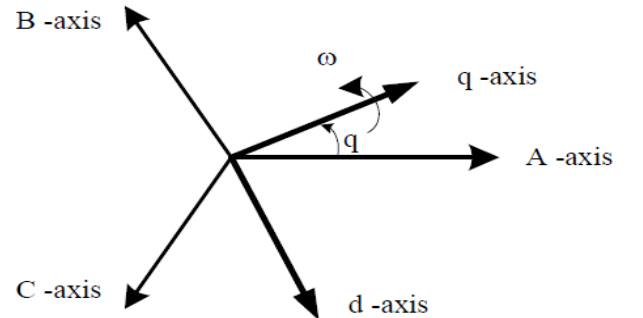
Fig..3. Change of variables 3Φ to 2Φ conversion
