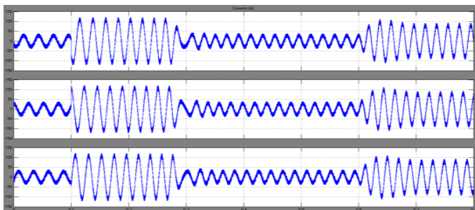
Fig. 15. Currents Response of Induction Motor Under Normal Condition
