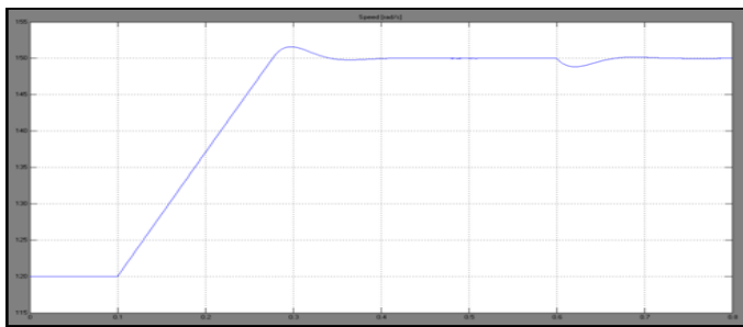
Fig. 13. Speed Response of Induction Motor Under Normal Condition
