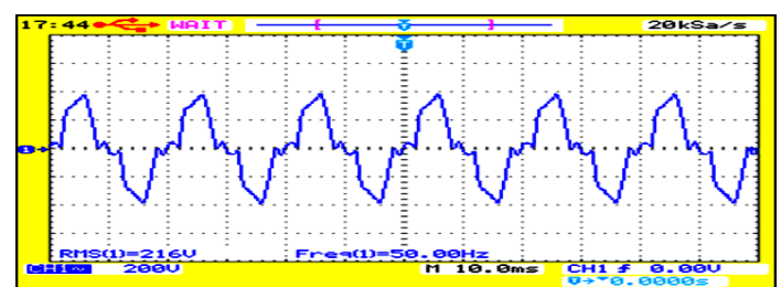
Fig. 21 Experimental Result for Voltage under Single Phasing Condition
