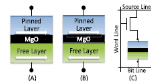
Fig. 1. Illustration of an MTJ and STT-RAM cell.
