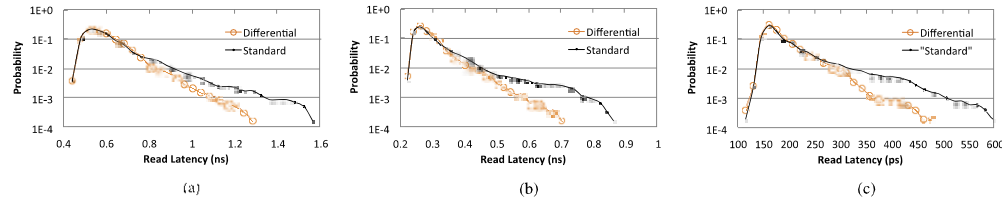
Fig. 6. Sense amplifier latency distribution to ensure <10^{-4} read error rate due to violating required delay (a) 45 nm. (b) 32 nm. (c) 22 nm.
