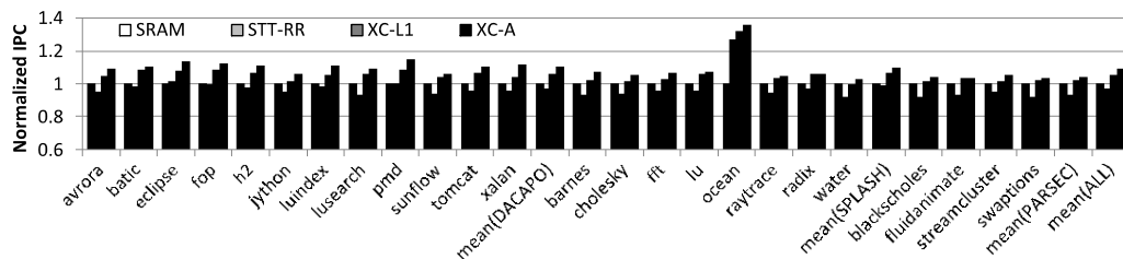
Fig. 9. Performance (IPC) comparison of SRAM and STT-RAM with X-cache (normalized to SRAM).
