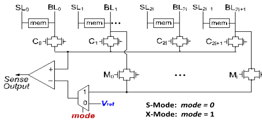
Fig. 7. Reconfigurable extreme mode (X-mode) memory circuit.
