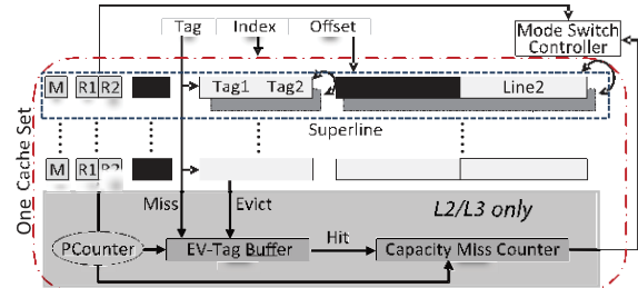
Fig. 8. Configurable cache architecture (X-cache).
