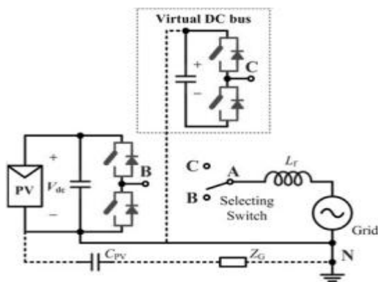
Fig. 9. Virtual DC Bus Concept Circuit.
