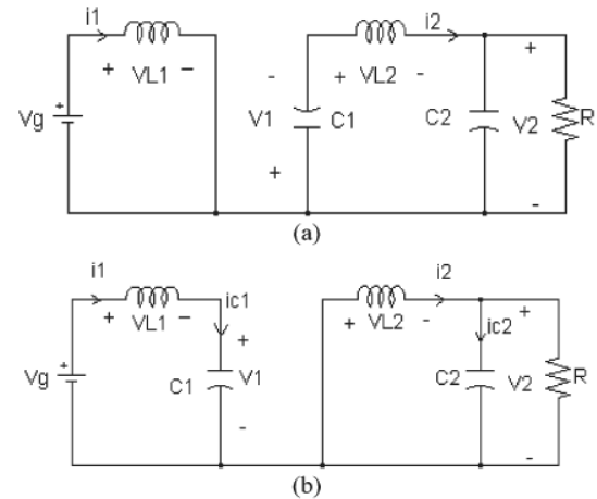
Fig. 7. Operating modes of CUK Converter Circuit
