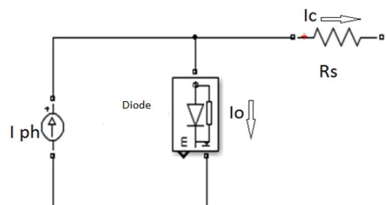
Fig. 2. Electrical Model of Photovoltaic Cell.
