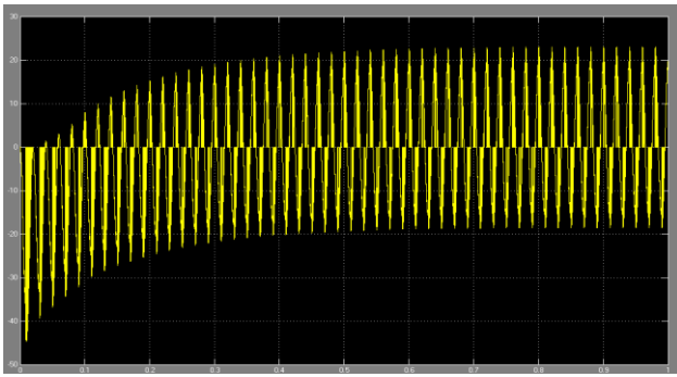
Fig. 17. Current Stress across Switches in H-bridge Inverter.
