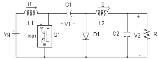
Fig. 6. Classical CUK Converter Circuit.
