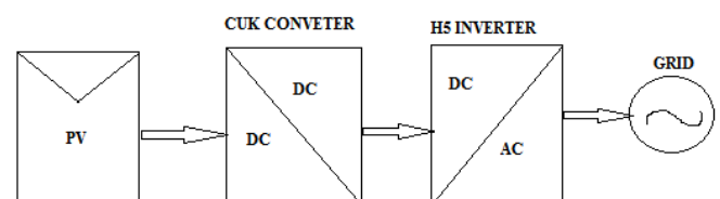
Fig. 1. Block diagram of the grid tied power system.
