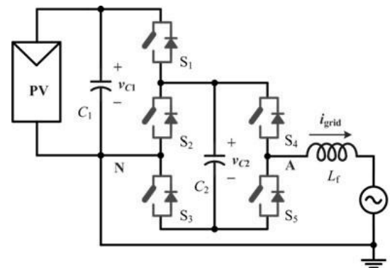
Fig. 10. Proposed H-bridge Inverter Topology Circuit.
