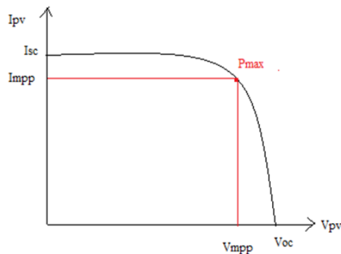
Fig. 3. Current Versus Voltage Characteristics of Photovoltaic cell.
