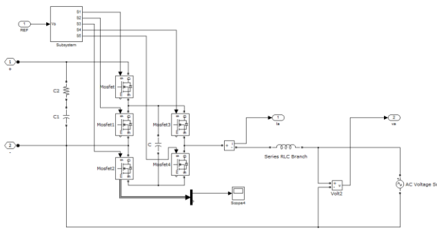
Fig. 12. Simulink Model of H-bridge Inverter.
