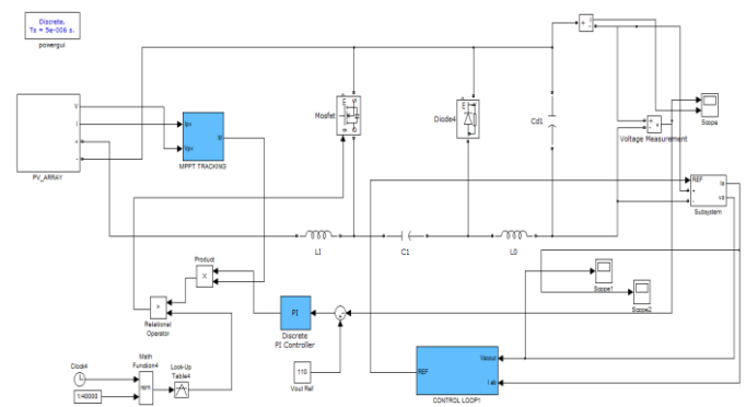
Fig. 11. Simulink Model of the grid connected system
