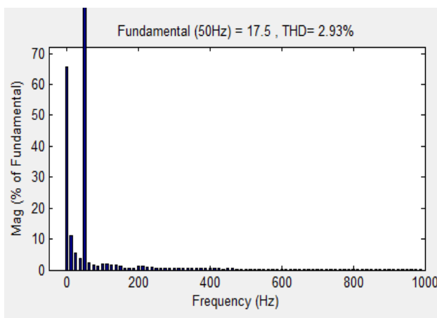
Fig. 20. THD of the Grid System.
