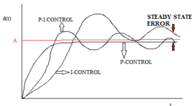
Figure 8. Comparison among the Transient Responses with P, I, P-I Controllers
