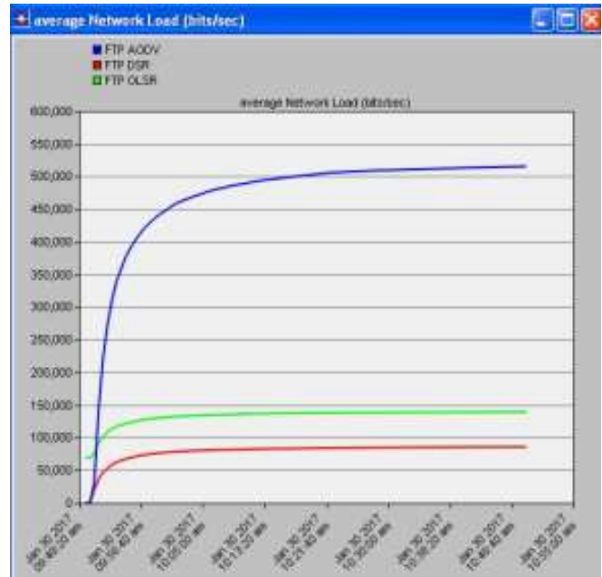
Fig. 6: Average Network Load
