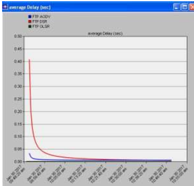
Fig. 5: Average End-to-End Delay
