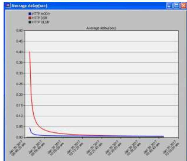
Fig. 2: Average End-to-End Delay
