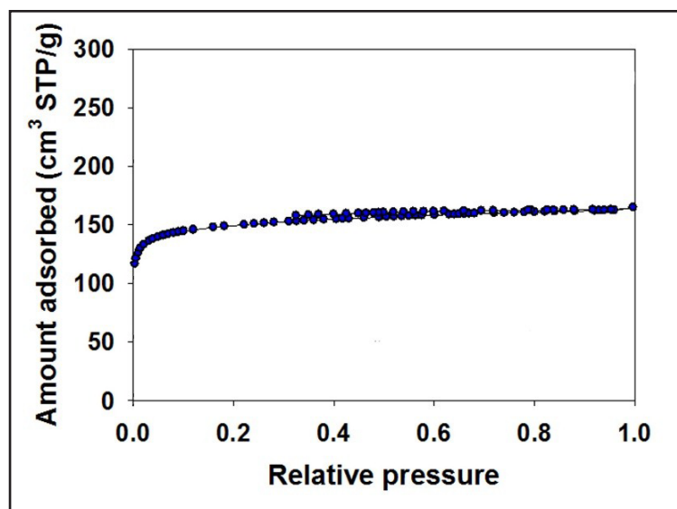
Fig. 1: Nitrogen Adsorption-Desorption Isotherms Curve
