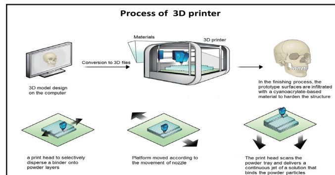
Fig. 2: Process of 3D Printing
