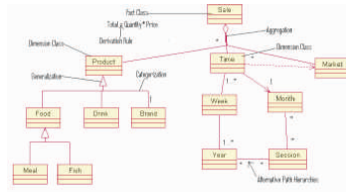
Fig 1 : OO Model of the Sale System
