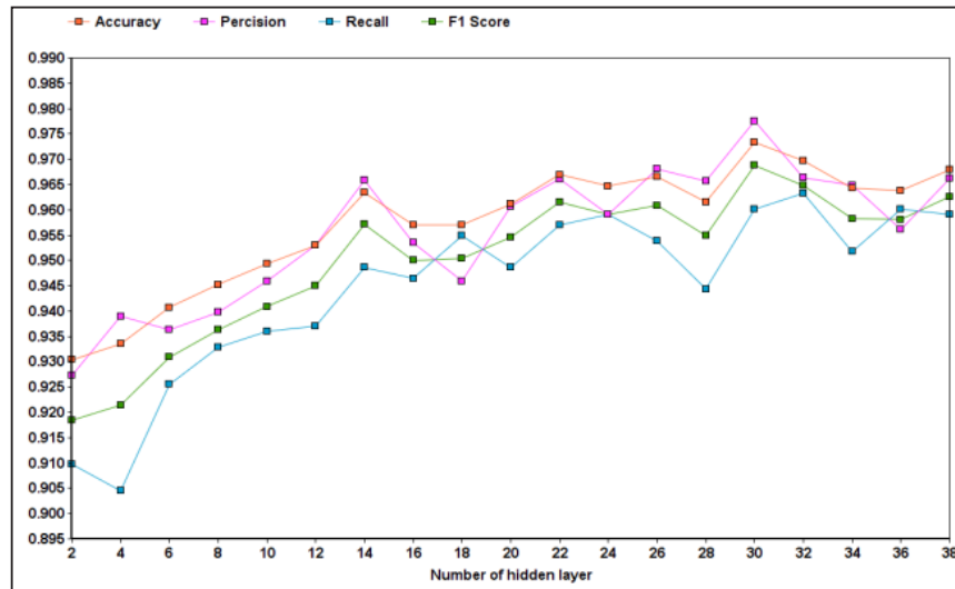
Fig. 7: Neural Network with Different Depth
