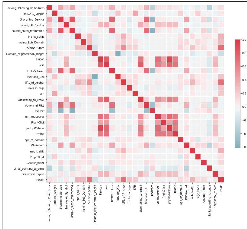
Fig. 4: Corrolation of Features in Datasets
