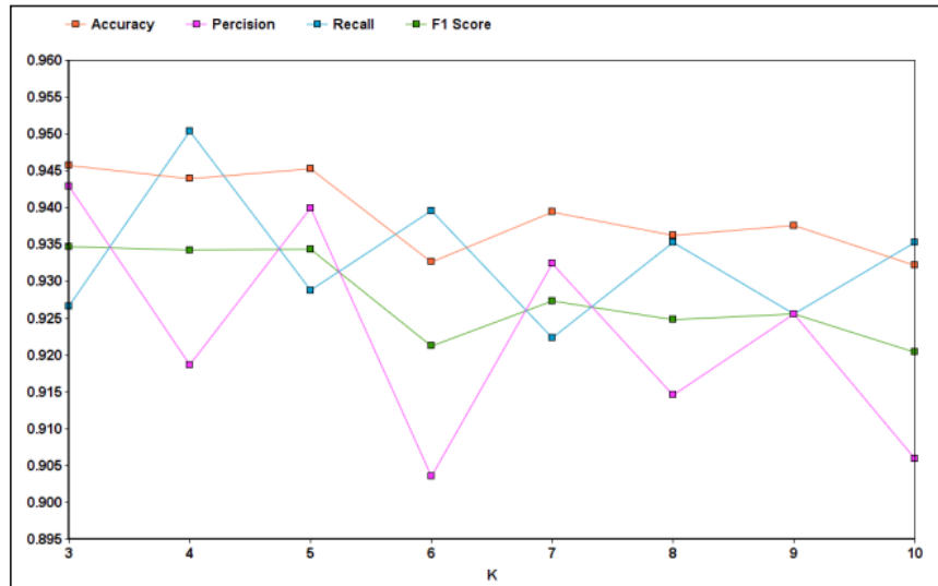
Fig. 6: KNN with Different K
