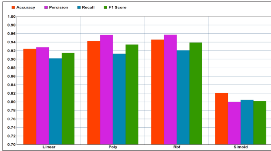
Fig. 5: Performance of SVM Classifier with Various Kernels
