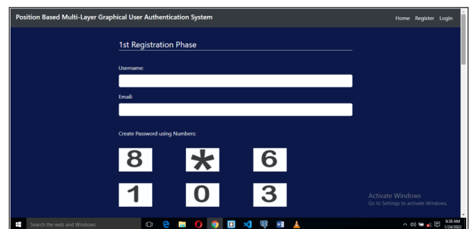
Fig. 4: Screenshot of Pegistration Page-Phase (Position-Based Multi-Layer GUAS)
