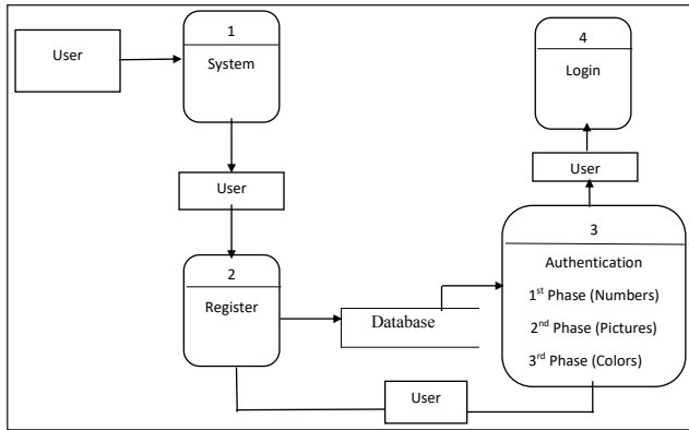
Fig. 1: Dataflow Diagram
