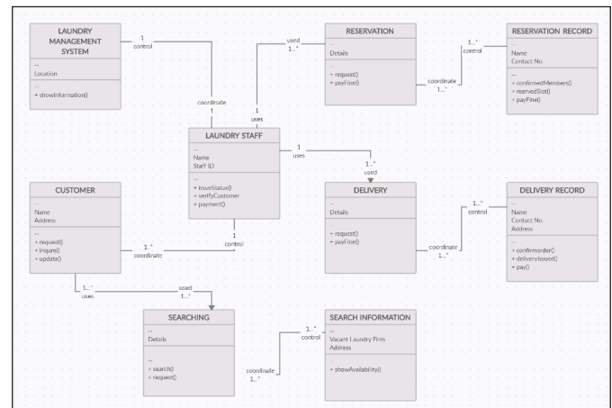
Fig. 10: Class Diagram
