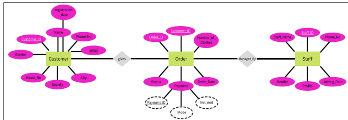
Fig. 9: Entity Relationship Diagram
